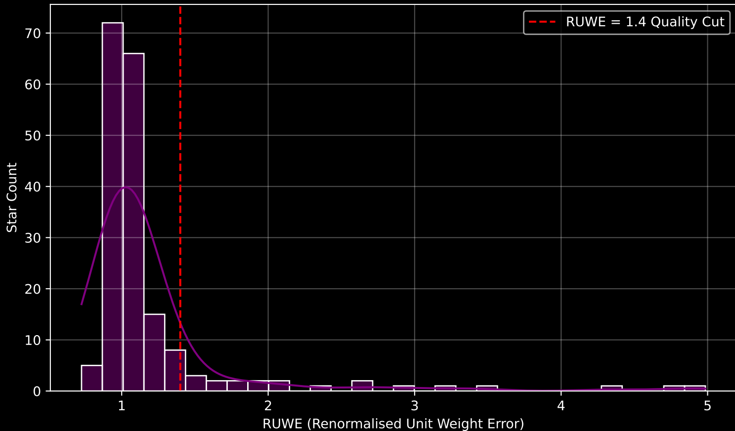
GAPOGEE DR17 Field [200+60] RUWE Distribution (n= 186)
