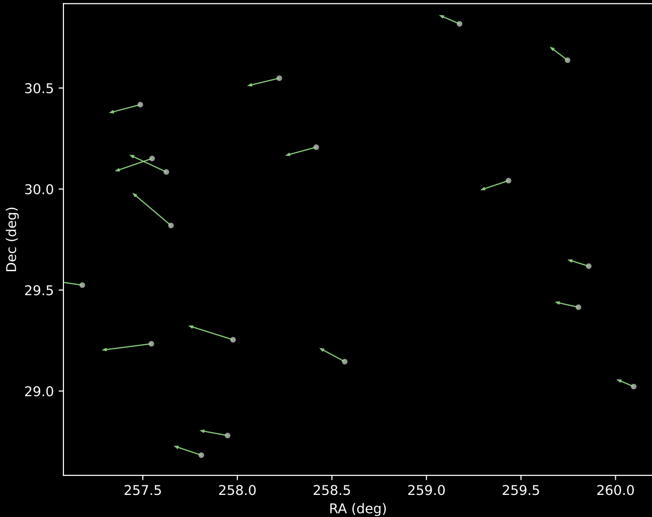
APOGEE DR17 Cluster 5 Proper Motion Vectors (n=18)
