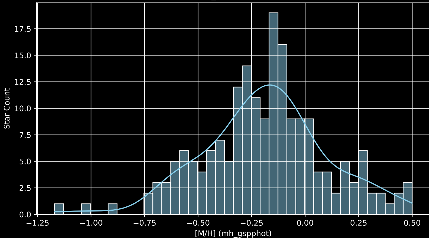
APOGEE DR17 Field: [200+60 [M/H] (mh_gspphot) (n= 191)
