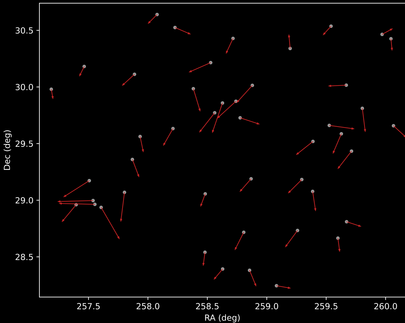
APOGEE DR17 Cluster 6 Proper Motion Vectors (n=45)
