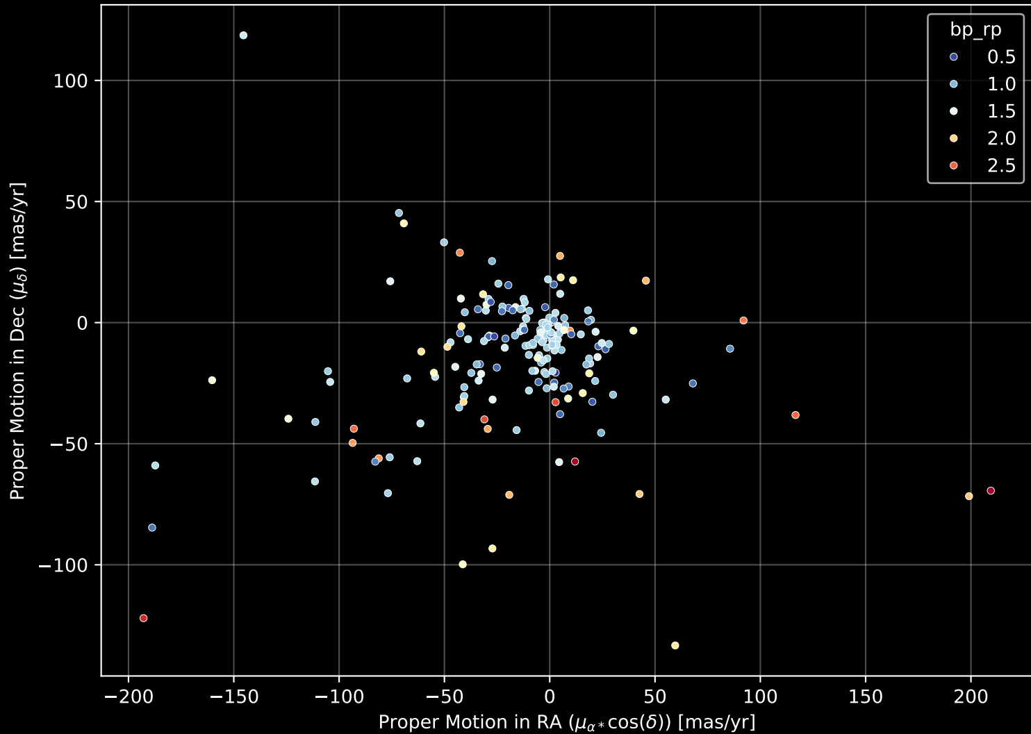
APOGEE DR17 Field: [200+60] Proper Motion Diagram (n= 195)
