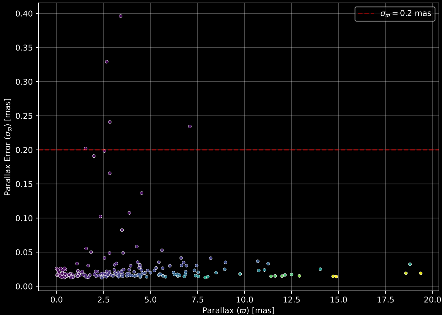
APOGEE DR17 Field: [200+60] Parallax Quality (n= 195)
