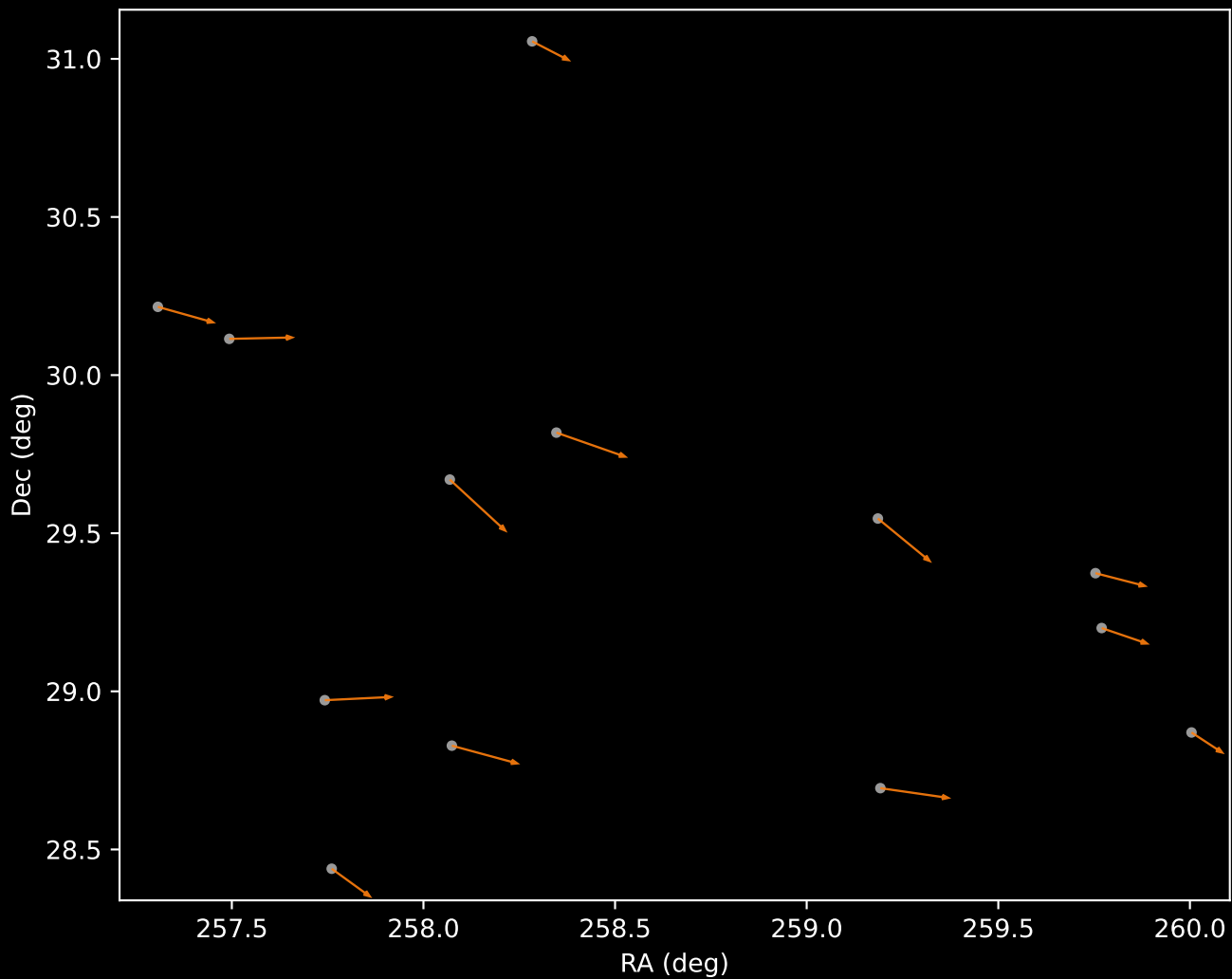
APOGEE DR17 Cluster 2 Proper Motion Vectors (n=13)
