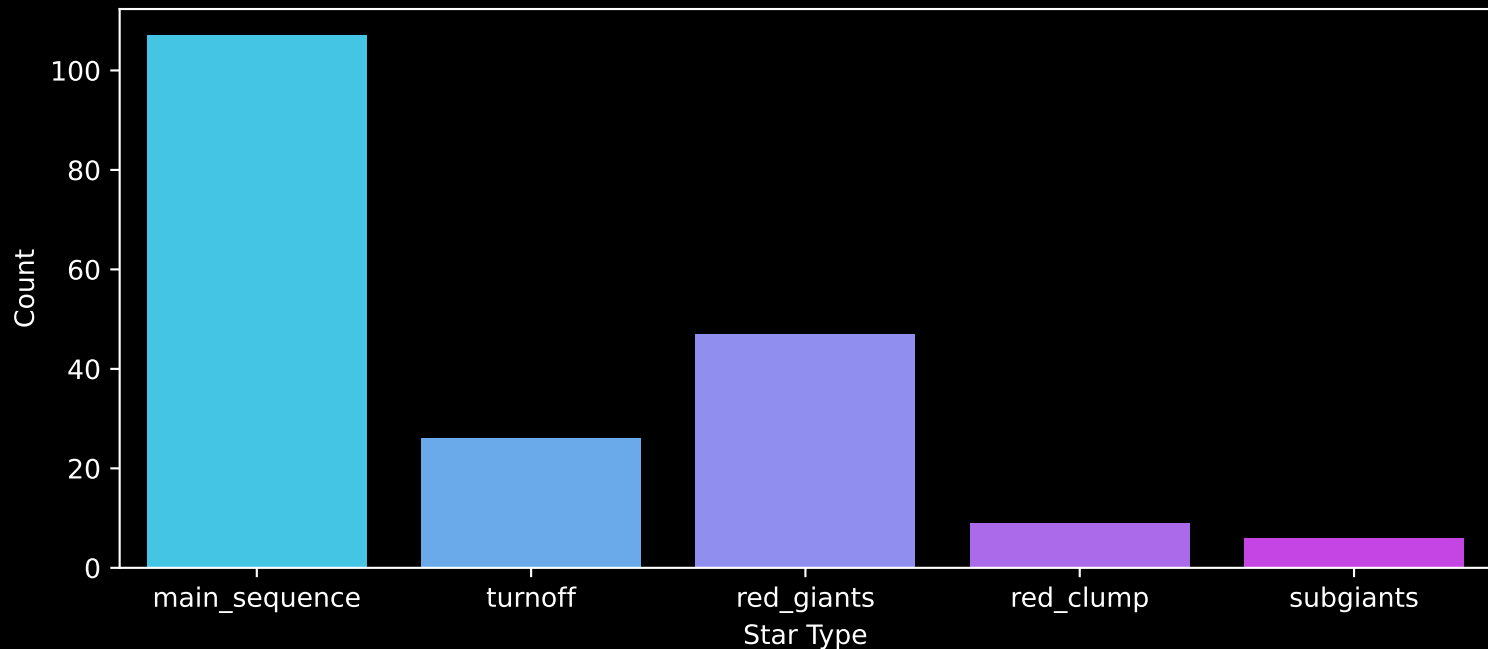
APOGEE DR17 Field: [200+60] Count plot of Star Type
